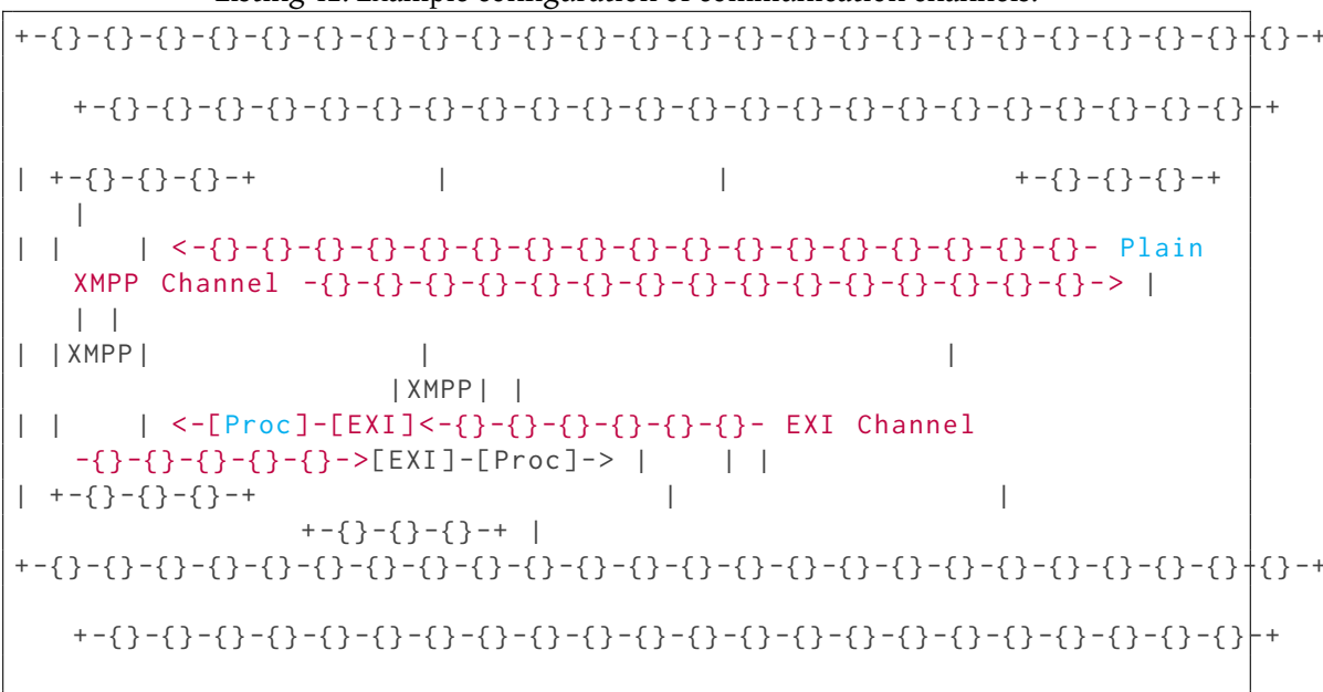
Listing 42: Example configuration of communication channels.
